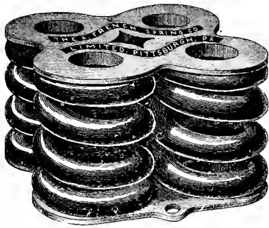
Fig. 5205. BOLSTER-SPRING. Four single-coil springs. Diameter of case, 11 ins. Height, 6 ins. Capacity, 6 to 8 tons.
